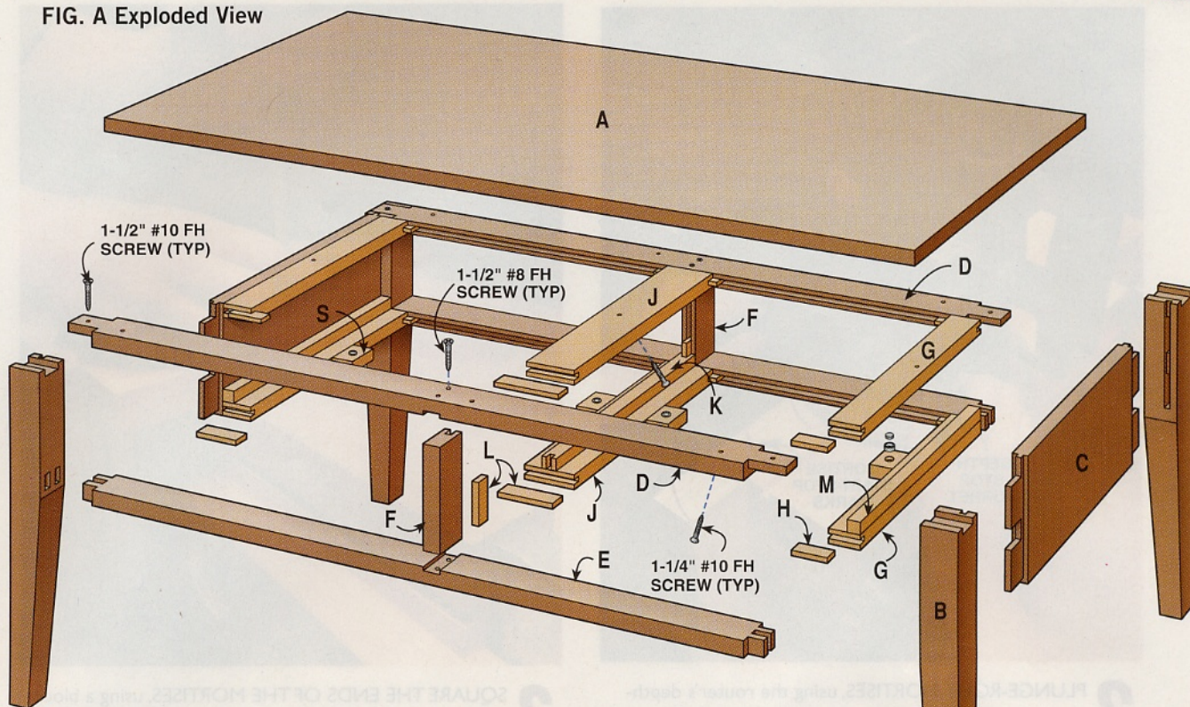
FIG. A Exploded View
