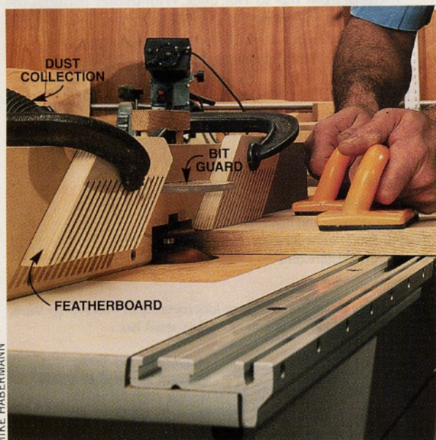
Photo 1 Featherboards, bit guards and dust collection allow you to safely do things with a router table that would be impossible with the router alone.
