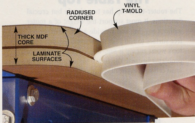
Photo 9 The best MDF tops are at least 1-1/16-in. thick and faced on both sides with high-pressure plastic laminate for a slick, durable, sag-resistant surface. Vinyl T-molding protects the raw MDF edges and radiused corners protect you when you back into them.
