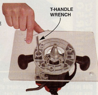
Adjust the bit's height without having to reach under your router table.
