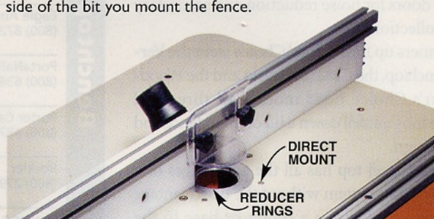
Photo 12 Direct mounting the router to the top creates an uninterrupted surface free of catch points caused by a mounting plate. Direct mounting also requires a much smaller hole, which results in a stronger top. On the downside, it's a hassle to remove the router for hand-held work.
