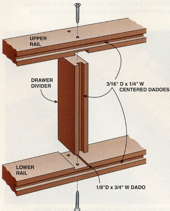
FIG. G Rail Dadoes
