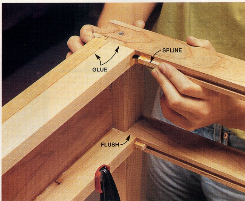
16 WOODEN SPLINES ALIGN THE RUNNERS AND RAILS PERFECTLY, just like a tongue-and-groove joint.
