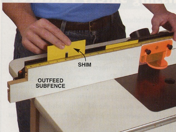
Photo 6 A subfence allows you to offset the outfeed fence with shims for edge jointing. Some manufacturers include shims, but you can easily make your own from paper, cardboard or plastic laminate.
