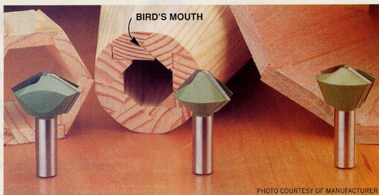
Bird’s-mouth joints lock staved pieces together.
