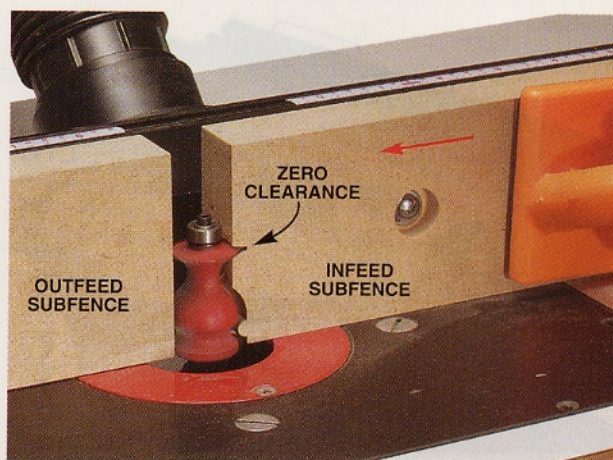
Photo 5 An adjustable sacrificial subfence is a must-have feature. The subfence allows you to adjust the fence opening to accommodate any sized bit. With the main fence secure, you can even push the infeed fence into a spinning bit and create a zero-clearance opening to eliminate chip-out.
