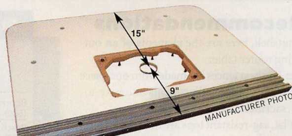
Photo 11 An offset router mount, when combined with a dual-position fence, allows you to choose the amount of table support between you and the router depending on which side of the bit you mount the fence.
