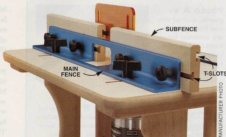
Photo 7 T-slots in the subfence work great, but in order to make your own subfence, you'll need to purchase a specialized router bit ($25). We prefer the easy-to-make subfence shown in Photos 4 and 5.
