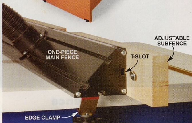
Photo 4 Here's what to look for in a router-table fence: Edge clamps allow you to position the fence anywhere on the table. A one-piece main fence doesn't have the alignment hassles of a two-piece fence. T-slots make convenient attachment points for subfences and accessories.
