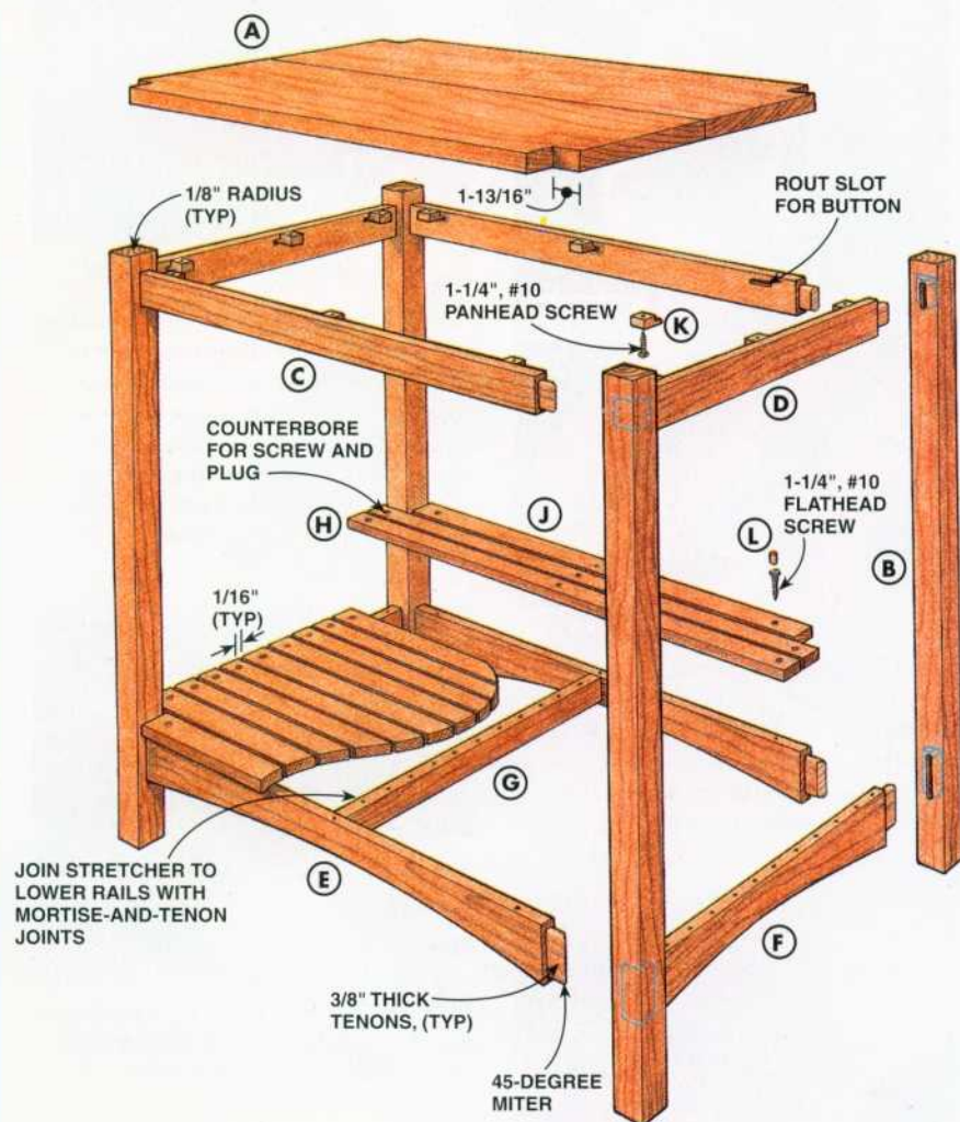
FIG A: Exploded View
