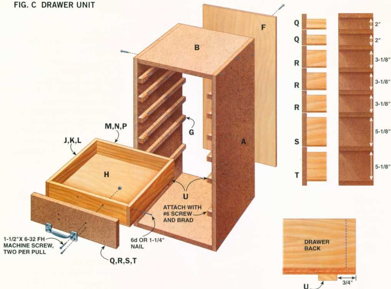
FIG. C DRAWER UNIT
