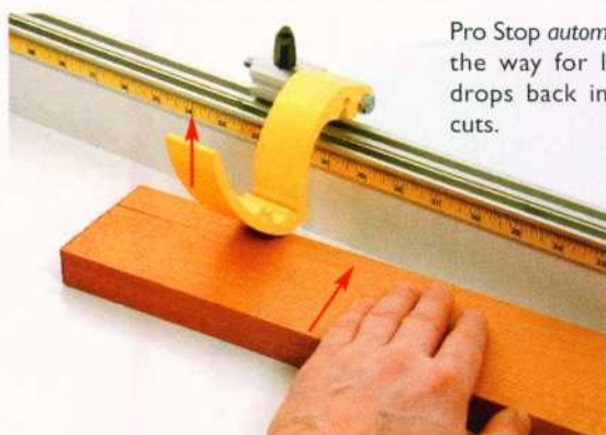
You can square boards and cut them to length without having to flip the stop each time by hand.
