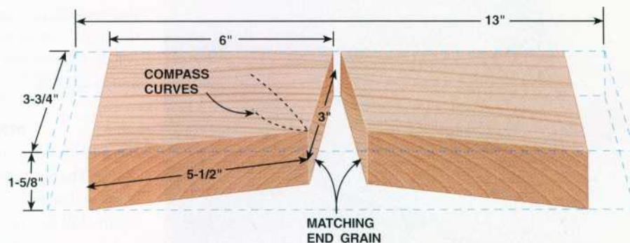
FIG. A Bookmatched Figure Create mirror images on the top of your bookends by cutting both core pieces from a single piece of wood. Lay out the angled sides of the blocks with a compass.
