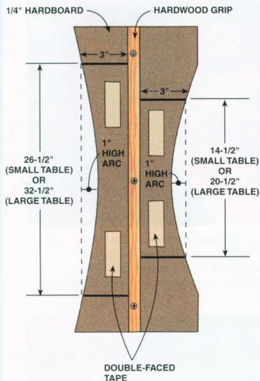
FIG B: Jig for Routing the Arched Rails
