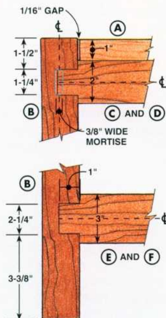
Detail 1: Apron and Rail Joints
