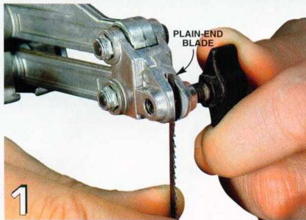
1 Tool-free blade clamping is the way to go. Most tool-free systems use a threaded knob to clamp the end of the blade in place.
