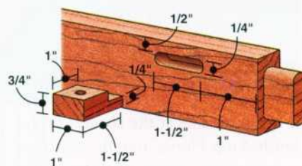
Detail 2: Slots and Top Fasteners
