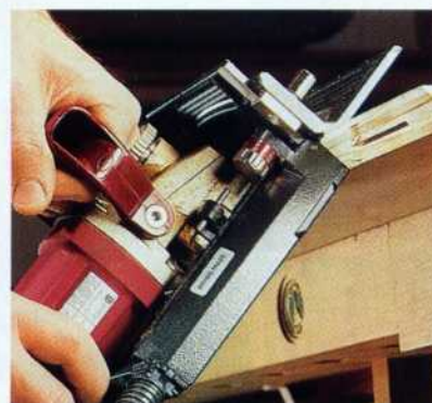
Cutting angle joints with a plate joiner is quick and easy. It's possible, but awkward, to do this with a router.
