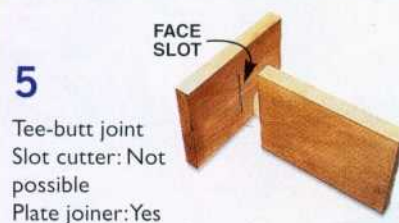
Cutting angle joints with a plate joiner is quick and easy. It's possible, but awkward, to do this with a router.
