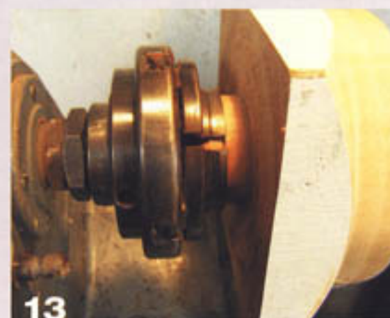
13 Remount the tenon of the newel post cap into a 4-jaw chuck using the turned groove as a marker for the teeth of the chuck.
