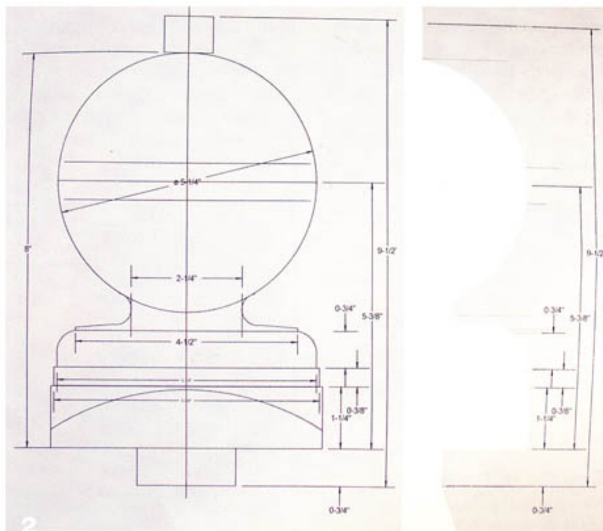
Drawing and template cutout.
