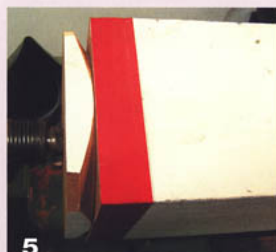
5 The shoulder is finished and it's time to turn the tenon.
