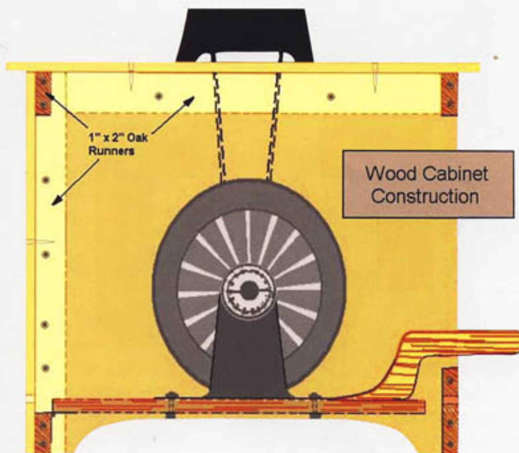
Diagram of the mobile lathe cabinet.
