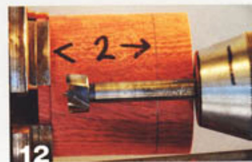
12 With the top section mounted in a chuck, mark the length for the top of the mill/shaker. Drill a \frac{3}{4} " (20mm) hole to a depth that will leave about \frac{1}{4} " (6mm) thickness on the top.
