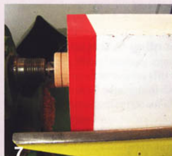
7 The tenon is finished and slightly rounded off at the bottom and there is a slight undercut to the shoulder.
