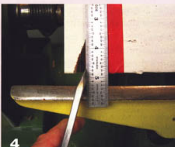
4 Cut with the skew chisel's right bevel parallel to the shoulder to create a square shoulder.
