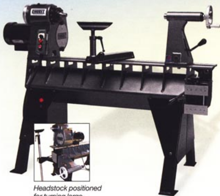
Robust 25 lathe
