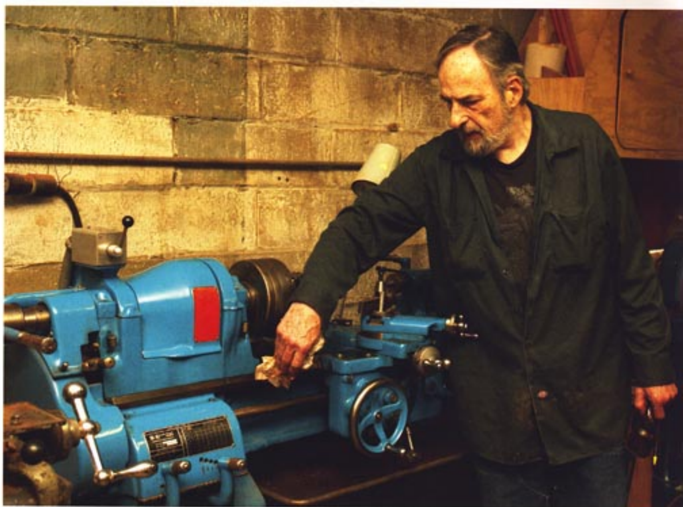
Giles with one of the lathes he lovingly restored, a 13" South Bend.
