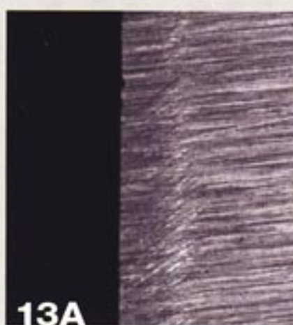
13A Cutting edge of a M2 HSS skew, ground and honed (200X).
