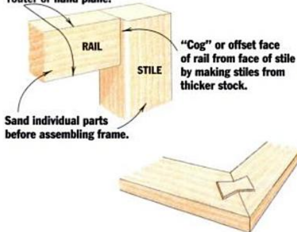
COGGED BUTTERFLY SPLINE
