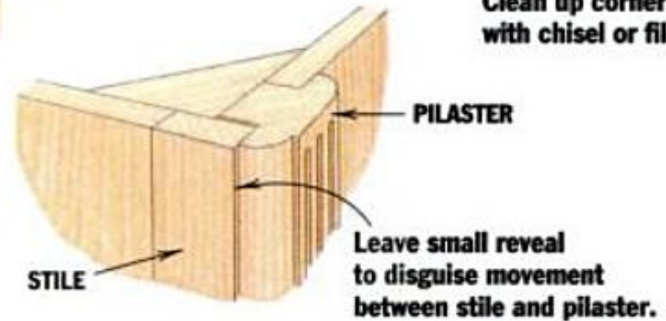
CARCASS CORNER
