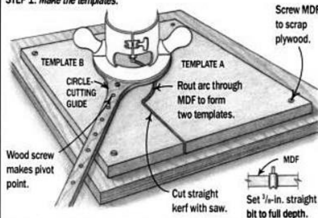
FIG. 2: MAKING PATCHES WITH A ROUTER
