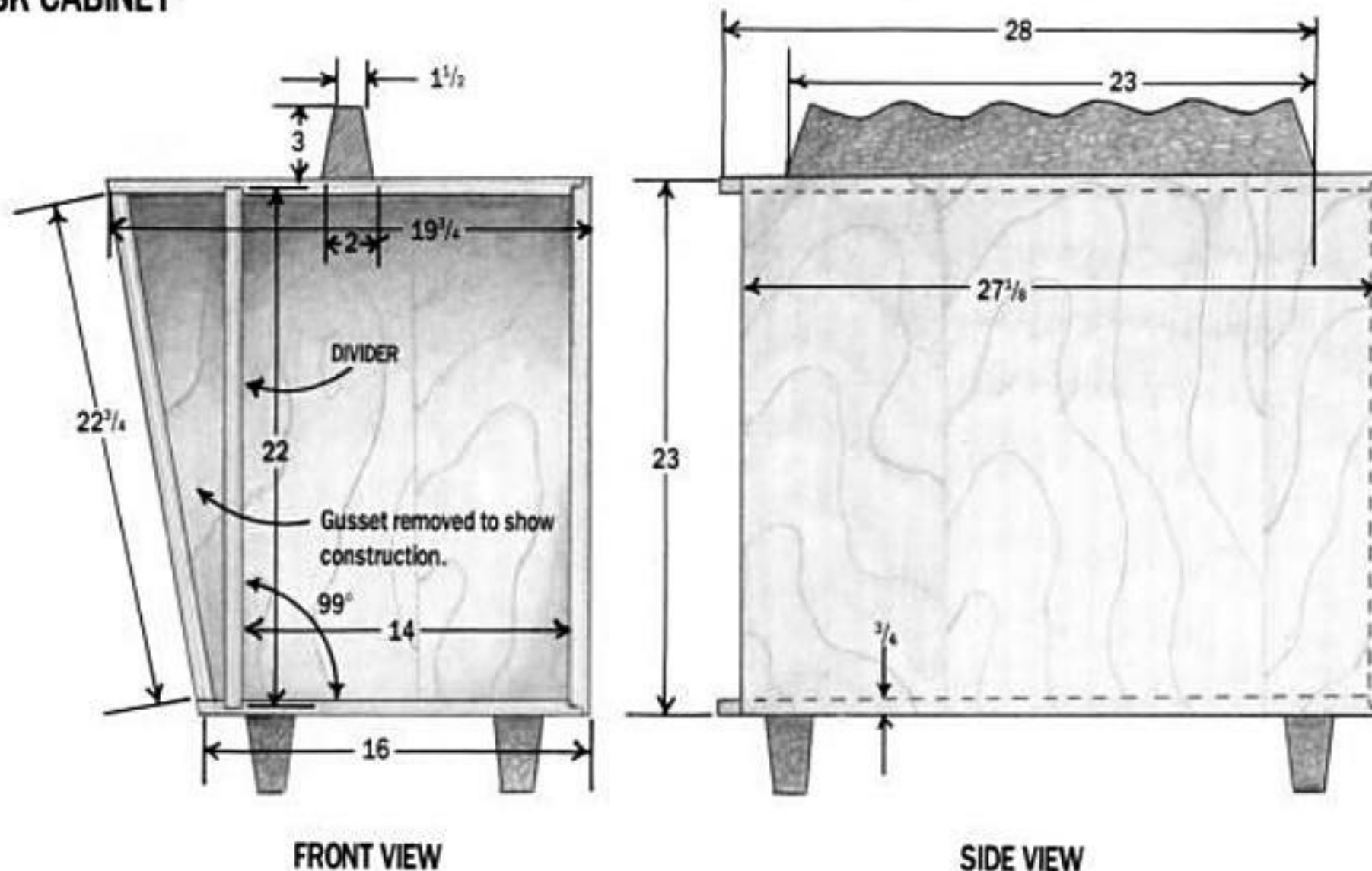
FIG. 3: DESK CABINET
