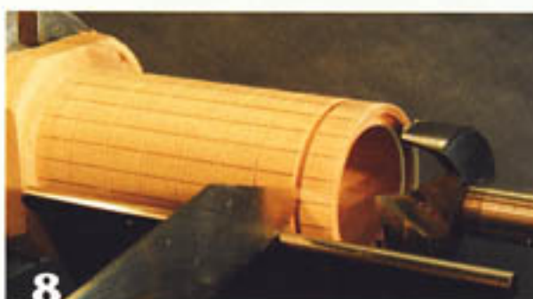
Using a thin parting tool, part off the first ring at the previously marked point. You should end up with a ring that is about \frac{3}{8} " (10mm) wide.
