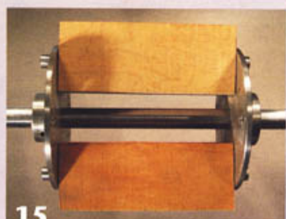
15 Two 3" x 3" x 9" (75mm x 75mm x 230mm) workpieces are mounted to the jig and are ready for initial turning.
