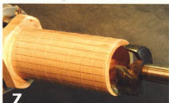
With a 1\frac{1}{4} " (45mm) Forstner bit mounted in a Jacobs chuck, drill \frac{1}{8} " (3mm) deep into the end of the tube to form a rabbet.
