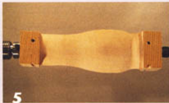
5 One of the workpieces has been remounted and is ready for turning between centers. Notice that the unturned ends have been trimmed.
