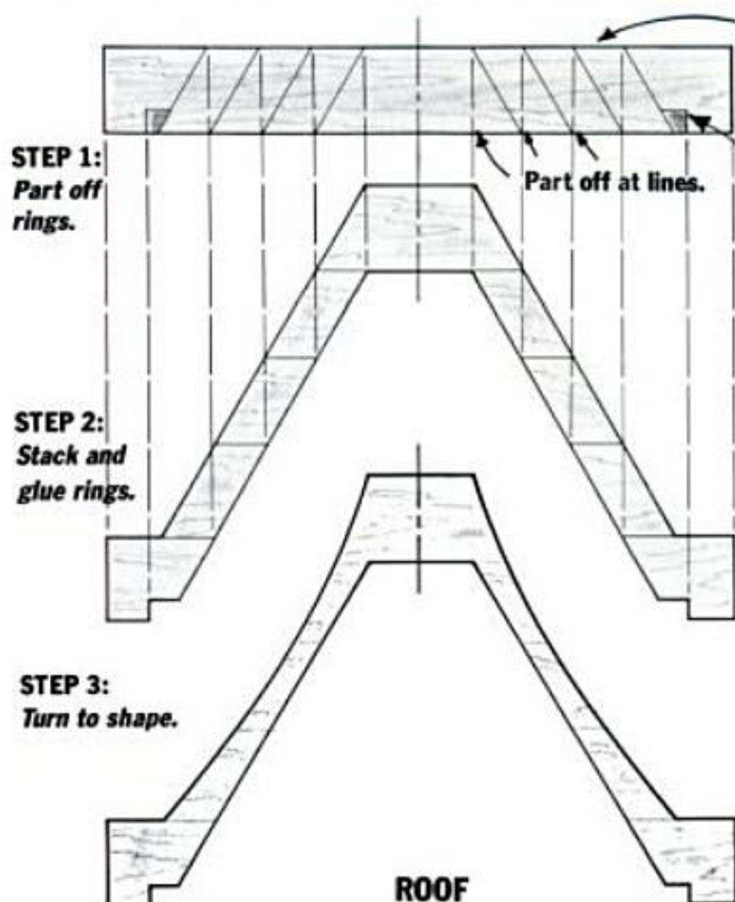
FIG. 2: CONSTRUCTING THE ROOF AND BASE
