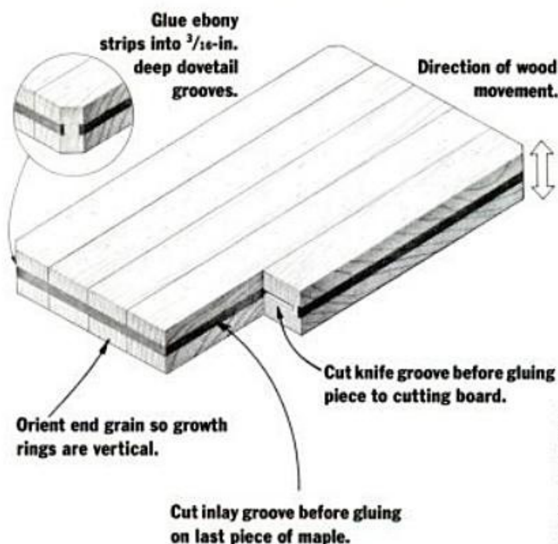
FIG. 1: LAMINATED CUTTING BOARD
