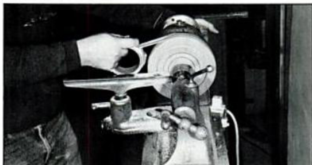
If you find the outside ring is rattling as you turn, tape it to the waste block.
