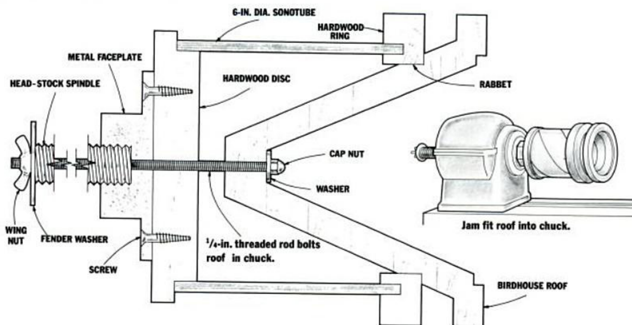
FIG. 4: CHUCK FOR TURNING INSIDE OF ROOF
