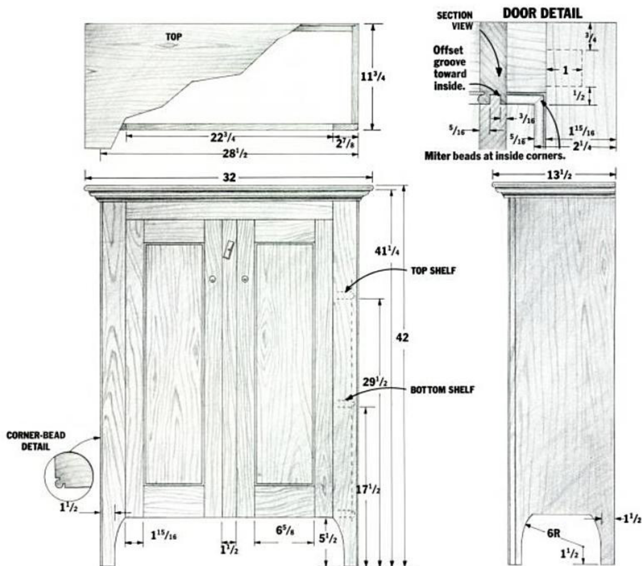
FIG. 1: NEW ENGLAND PINE CUPBOARD
