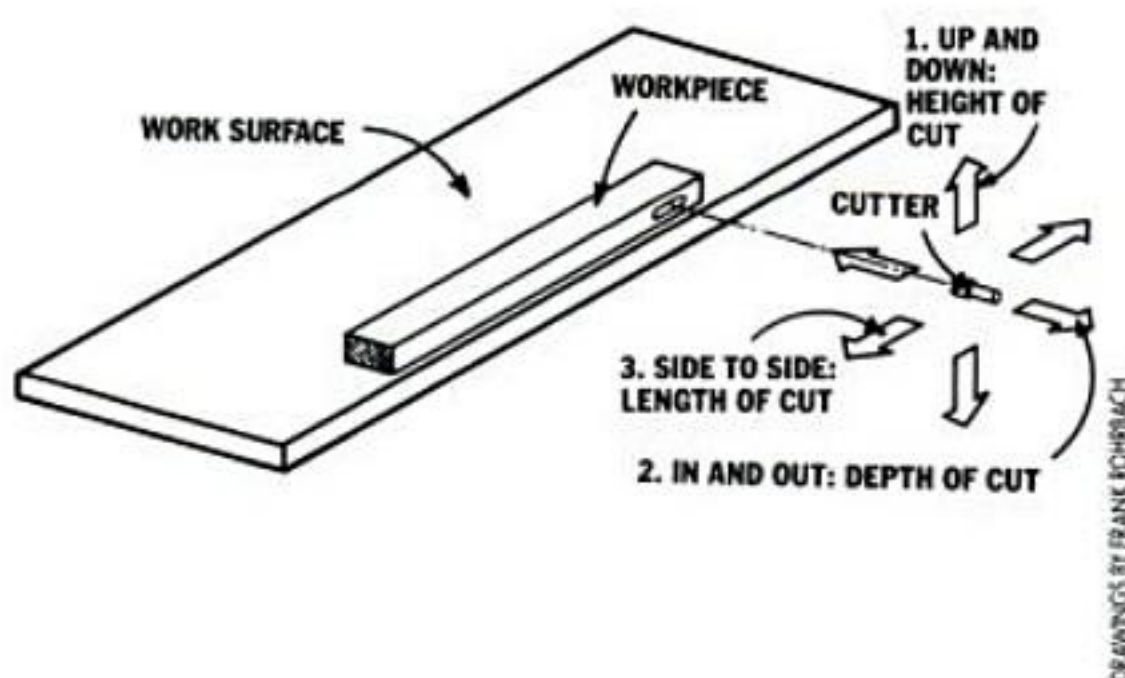
FIG. 1: THREE AXES OF MOVEMENT OF A SLOT MORTISER
