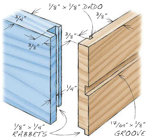
Fig. C Drawer Details
