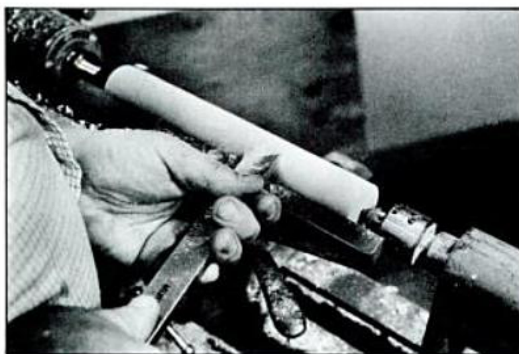
The planing cut shaves the long-grain surface smooth. Hold the skew long point up and angle the tool slightly in relation to the wood's axis. Cut between the center part of the edge and the short point, and keep the bevel rubbing as you cut.
