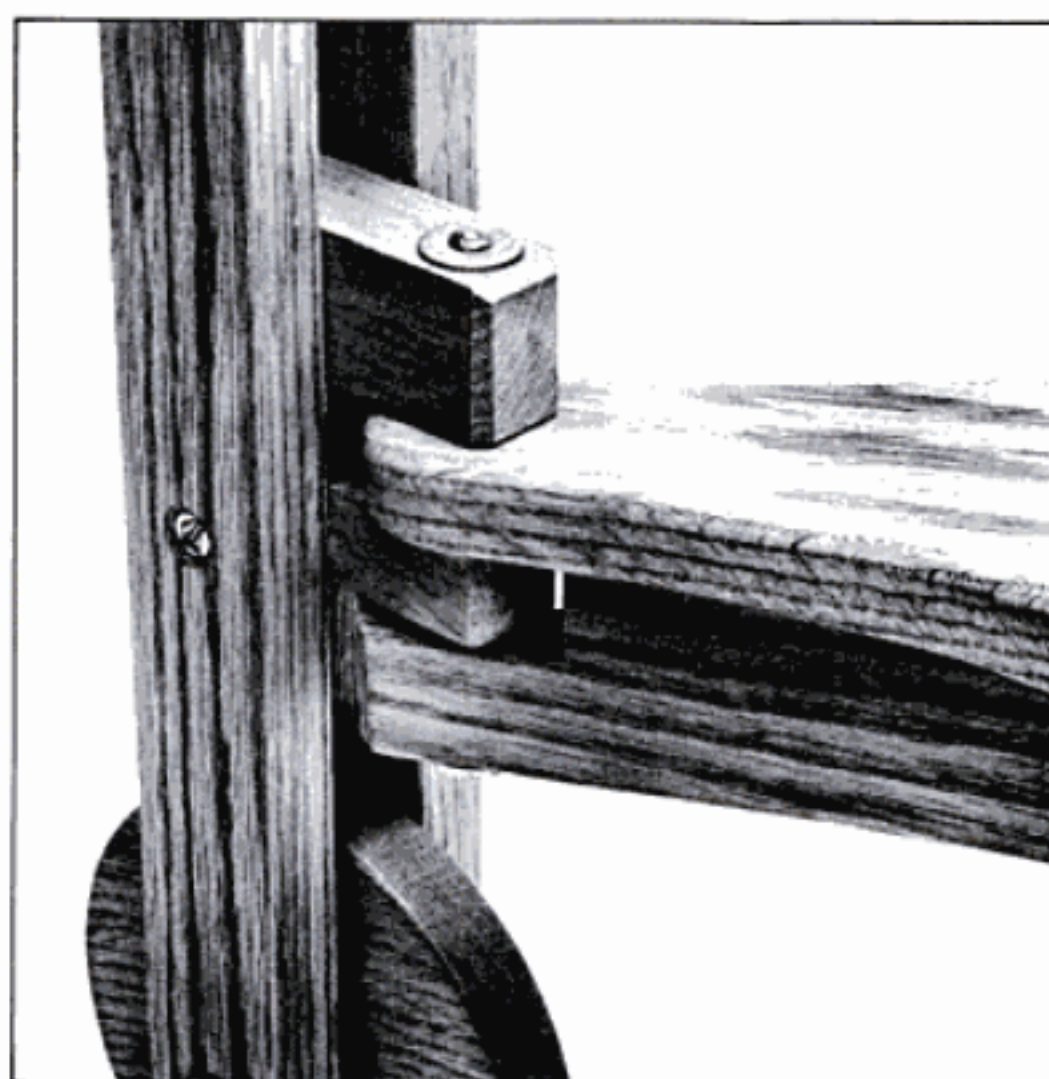
The steering assembly pivots on a \frac{5}{16} -in. dia steel rod through the seat.
