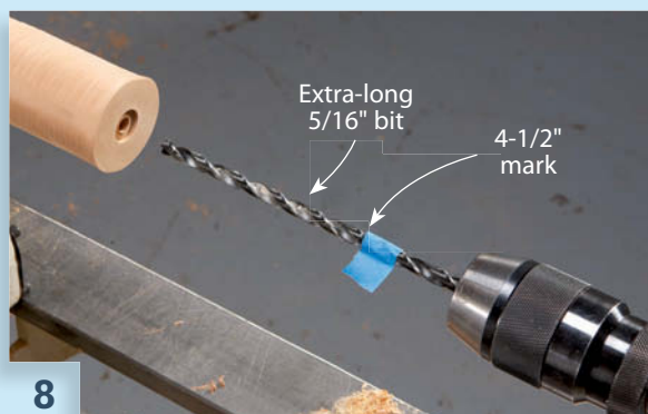
8 Continue drilling the hole with an extra-long 5/16" bit. Make this hole at least 4-1/2" deep.
