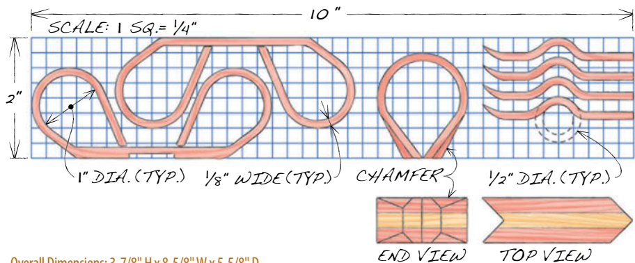
Fig. C Ribbon and Bow Pattern
