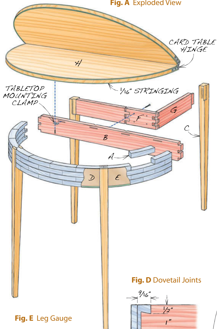
Fig. A Exploded View
