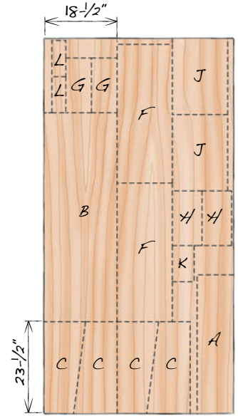
Fig. B Plywood Cutting Diagram
