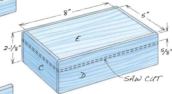
Fig. B Box Dimensions Before Sawing
