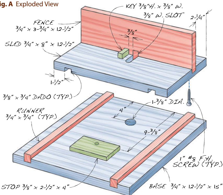
Fig. A Exploded View
