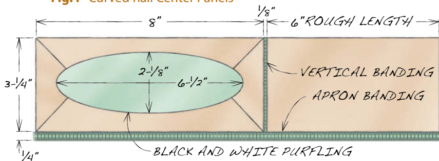
Fig. F Curved Rail Center Panels
