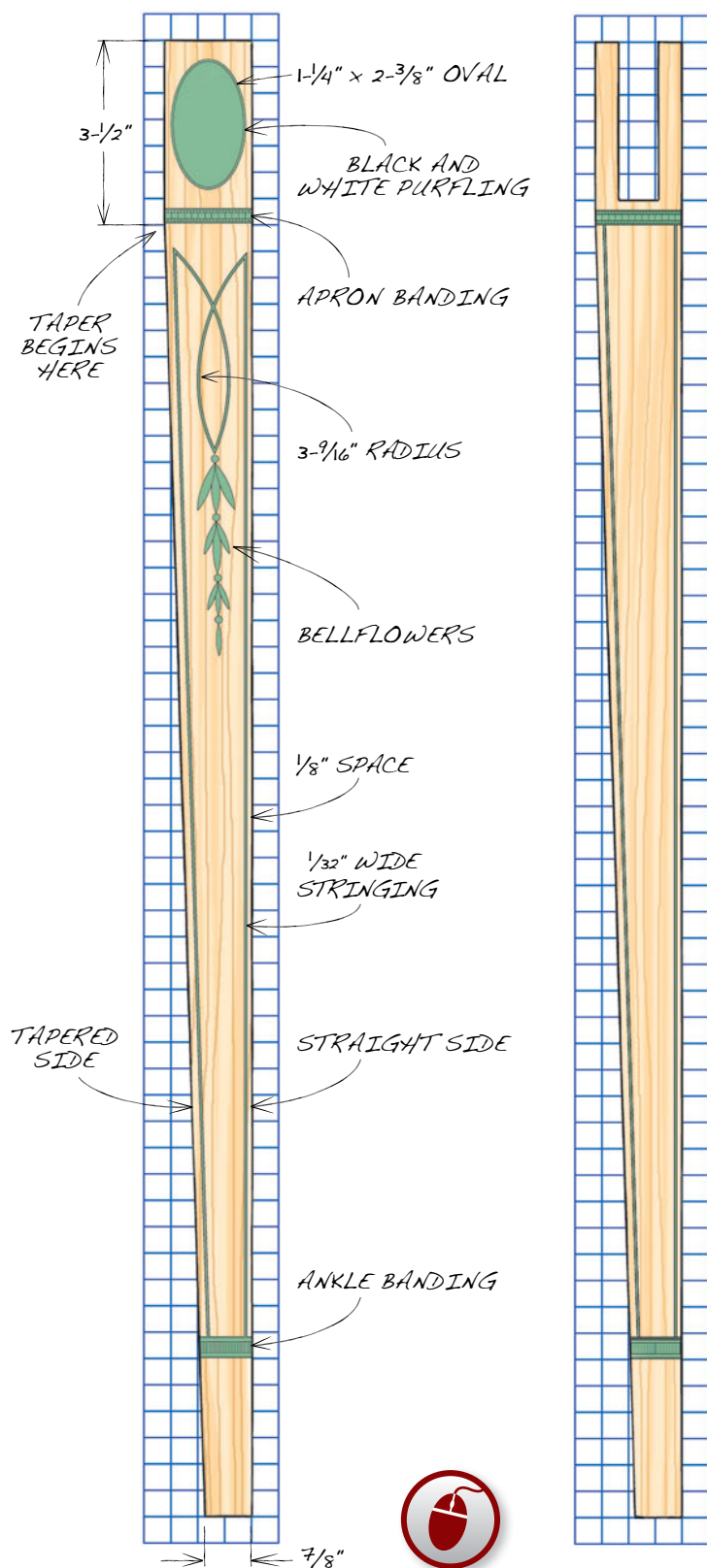
Fig. G Leg, Front and Side View
