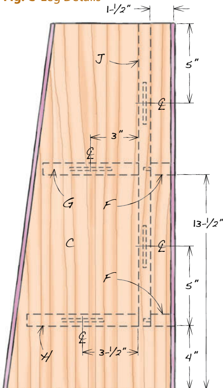
Fig. C Leg Details
