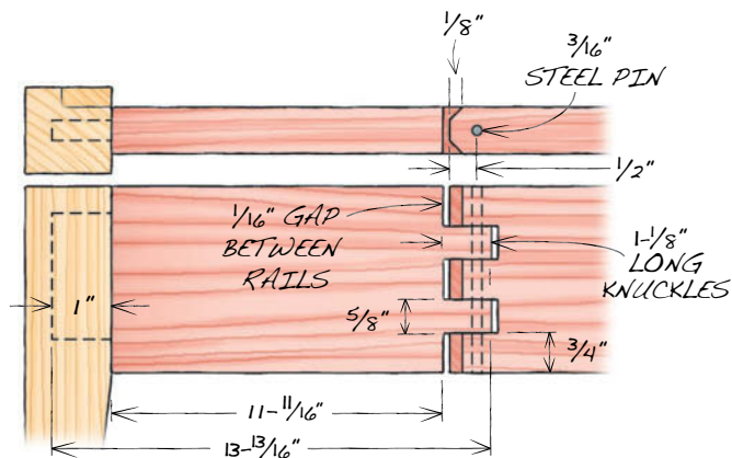
Fig. L Swinging Rail and Knuckle
