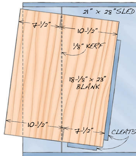
Fig. D B Leg Tapering Set-up
