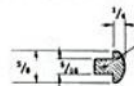
DOOR MOLDING PROFILE
