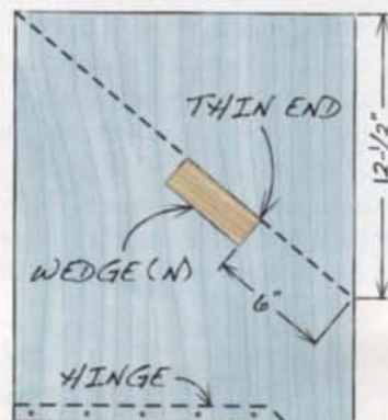
Fig. D Wing Support Pattern
