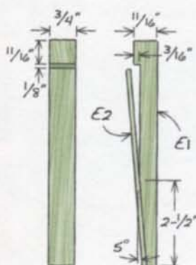
Fig. H Bench Dog
