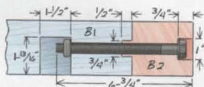
Fig. G Tail-vise Plate-setting Jig
