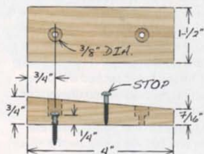
Fig. C Location of Wedge
