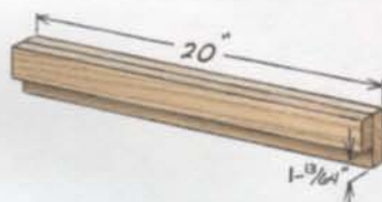
Fig. G Tail-vise Plate-setting Jig
