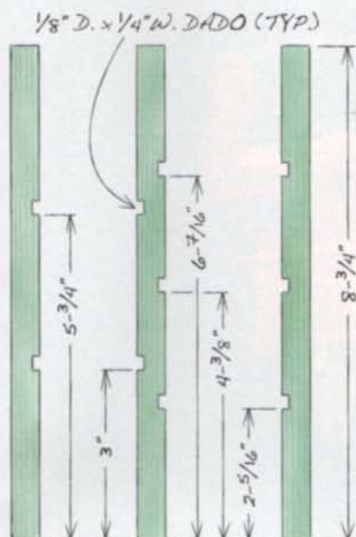
Fig. B: Drawer Dado Details
