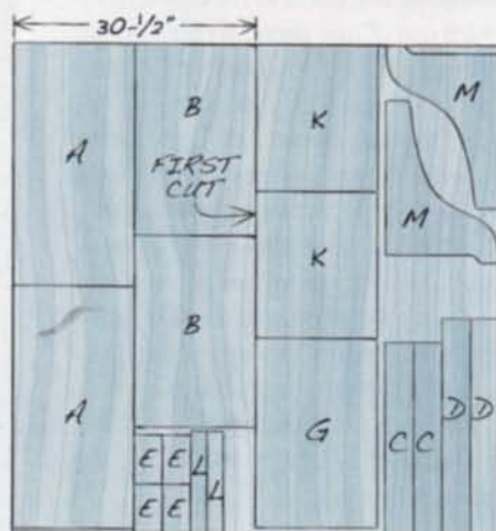
Cutting Diagram for 5' x 5' Baltic Birch
