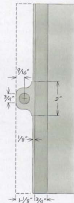
Fig. C: Drawer Pull Profile
