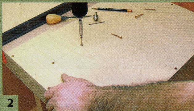
2 Attach a plywood sub-top to the base. The subtop prevents the base from racking. It also supports the working top which is made from 1/2" thick solid-surface material, such as Corian or Avonite.
