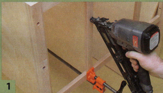
1 Begin building the router table by making the base. Construction is quite simple, using just screws, glue, and a nailed-on face frame in front.
