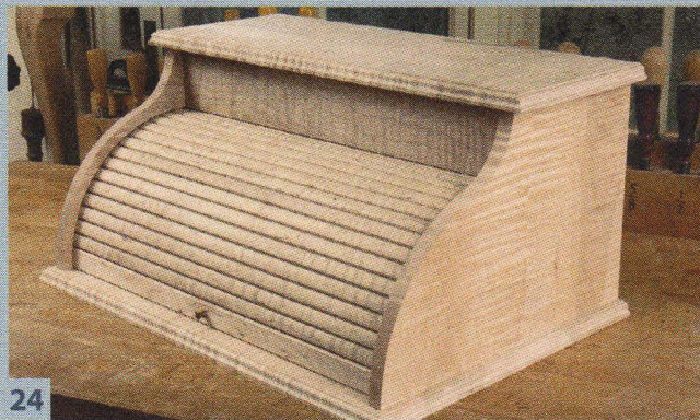
24 Make sure the door slides without binding, then remove the base. Disassemble the door so you can finish its pieces separately.
