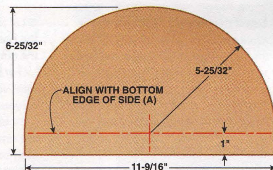
Fig. E Rear View and Underside of Top
