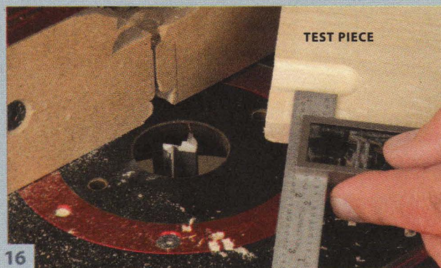
16 Using a bit that's the same width as the sides, make a test cut in a scrap piece to make sure the grooves are the correct distance from the edge.
