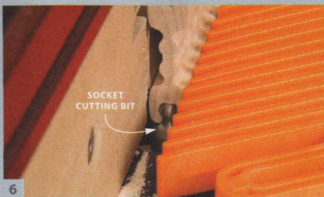
Finish the sockets on the router table.
