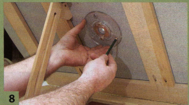
8 Drill a 3/4" dia. hole through the top, then remove the router's baseplate and mark the locations of its mounting holes onto the top. Drill the holes and lower the top.
