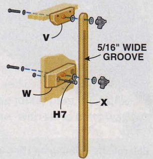
Fig. D Support Arm
