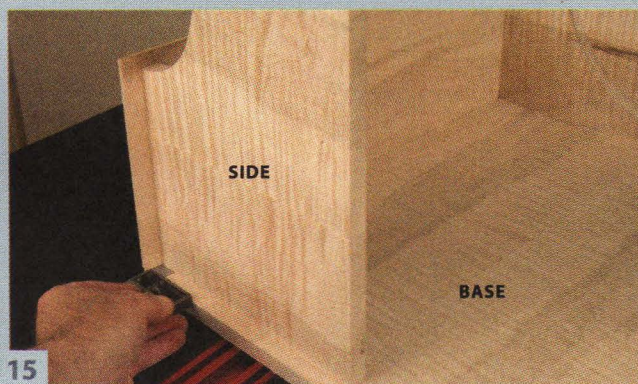
15 Assemble the top and sides temporarily. Center this assembly on the base in order to mark the location of stopped grooves that will receive the sides.
