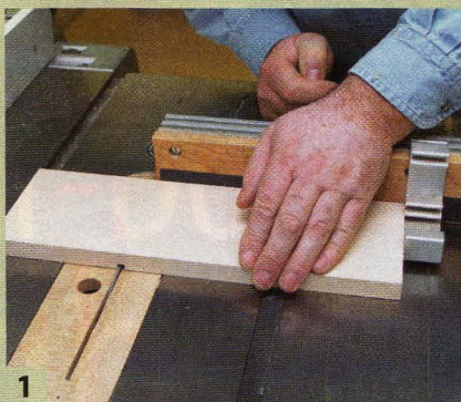
1 The caddy is held together with sliding-dovetail joints. Start by cutting dadoes in the sides to remove most of the waste.
