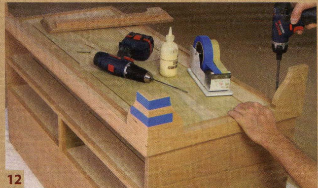
12 Fasten the base one piece at a time to the chest's bottom. This method guarantees a tight fit between the chest and the base's molding. Glue and tape the feet's mitered corners.
