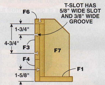
Fig. G End View of Fence
