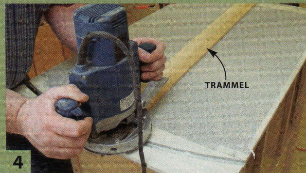
4 Rout an arc on one end of the solid-surface top using a trammel fastened to the router's base.
