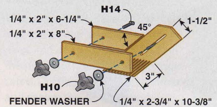
Fig. F Featherboard
