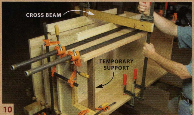
10 Add the front. It sits on the upper web frame, but needs support to stay square. Apply a small amount of pressure in the middle using a crossbeam. When this dries, add the remaining end.
