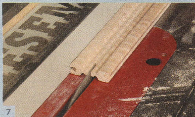
Rip each blank down the middle, creating two tambour slats.
