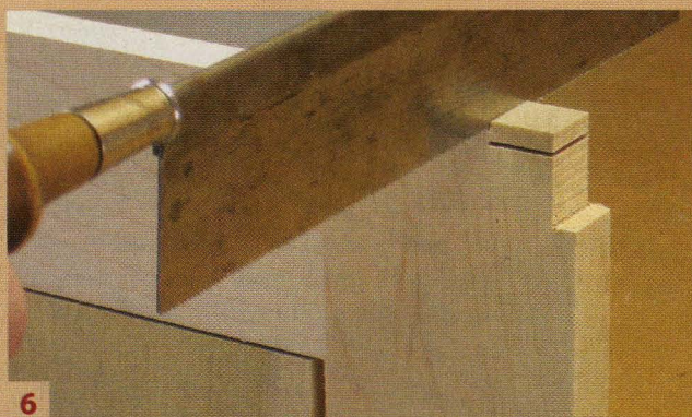
Cut notches on the rear corners of the web frames to fit the stopped grooves. Make the long cuts first using a bandsaw, then finish the cuts by hand.
