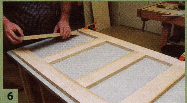
6 Build a frame to fit inside the rectangle you drew. Glue the frame to the top using silicone adhesive. Attach the top assembly to the case with a continuous hinge.
