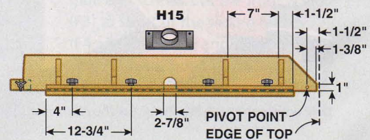
Fig. H Top View of Fence
