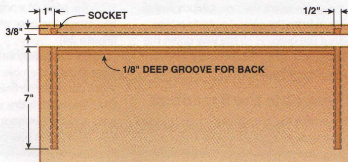
Fig. E Rear View and Underside of Top
