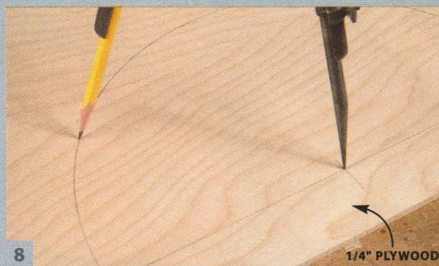
Begin building the case by laying out a semi-circular template. This will guide your router in making the grooves that house the tambour door.
